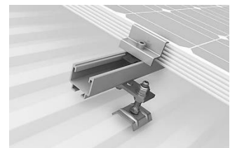
Z purlin farm roof fixing kits
