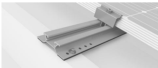
Mini rail corrugated roof fixing kits
