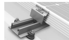
Trapezoidal roof fixing kits (metal box section clad)
